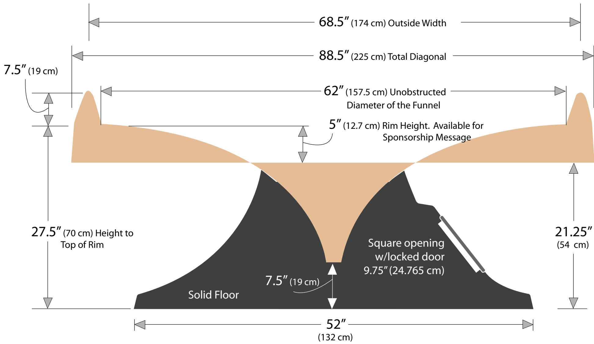
7' Sprial Wishing Well - Detail Divnick International
